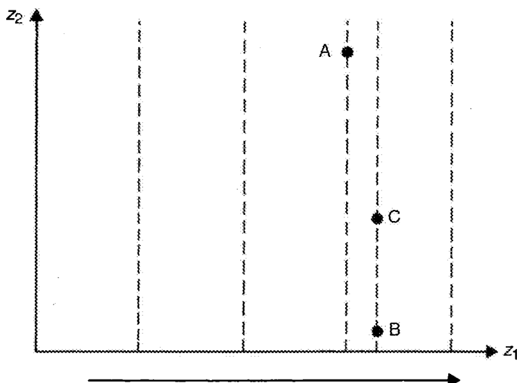
Figure 2.2 Naïve lexicographic ordering
